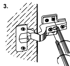
3. Tighten 2 screws in oval holes. Screw in 2 screws in round holes
