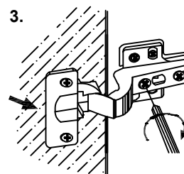
3. MOVE DOOR INWARD by turning this screw clockwise
