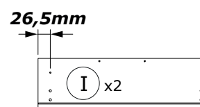
CS3259 593x180x18mm
